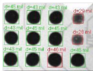
Ball Diameter Measurements
