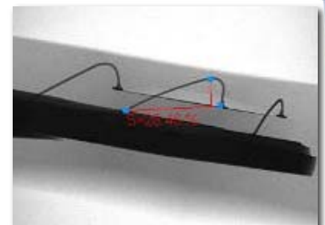
Wire Bond Measurements
